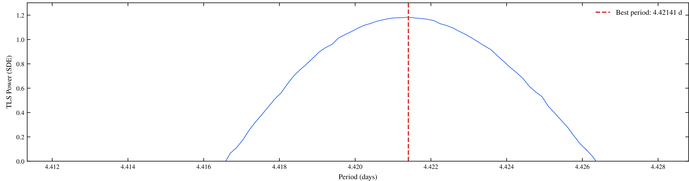
TIC 461867584 | Sectors: 36, 37 | TLS Fine Periodogram (SDE = 1.18)
