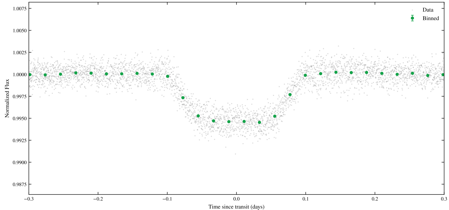
TIC 461867584 | Sectors: 36, 37 | Phase-Folded Transit (P = 4.42141 d)
