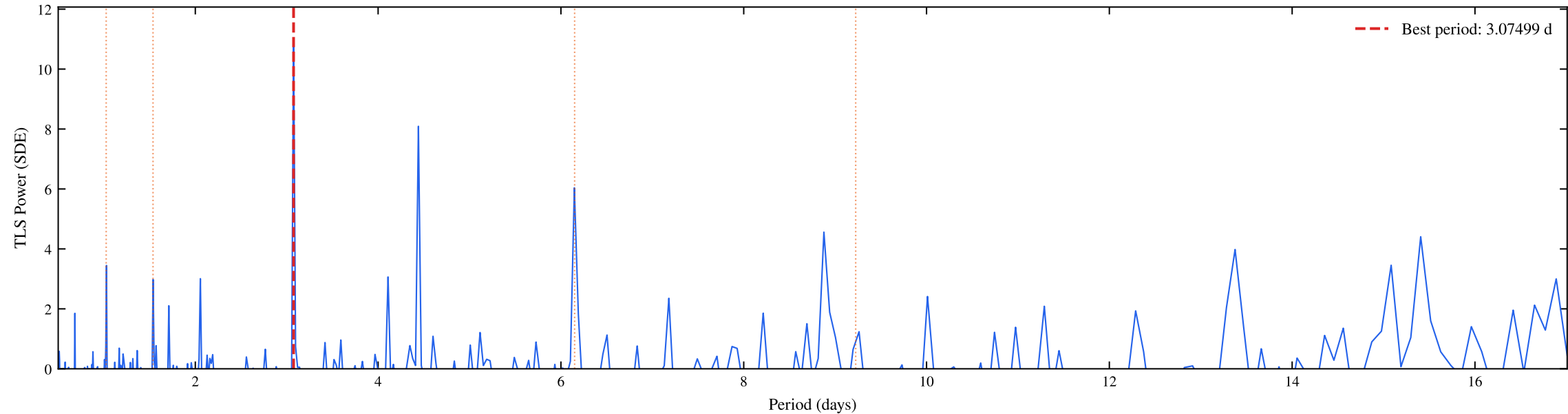
TIC 461867584 | Sectors: 36, 37 | TLS Coarse Periodogram (SDE = 10.97)
