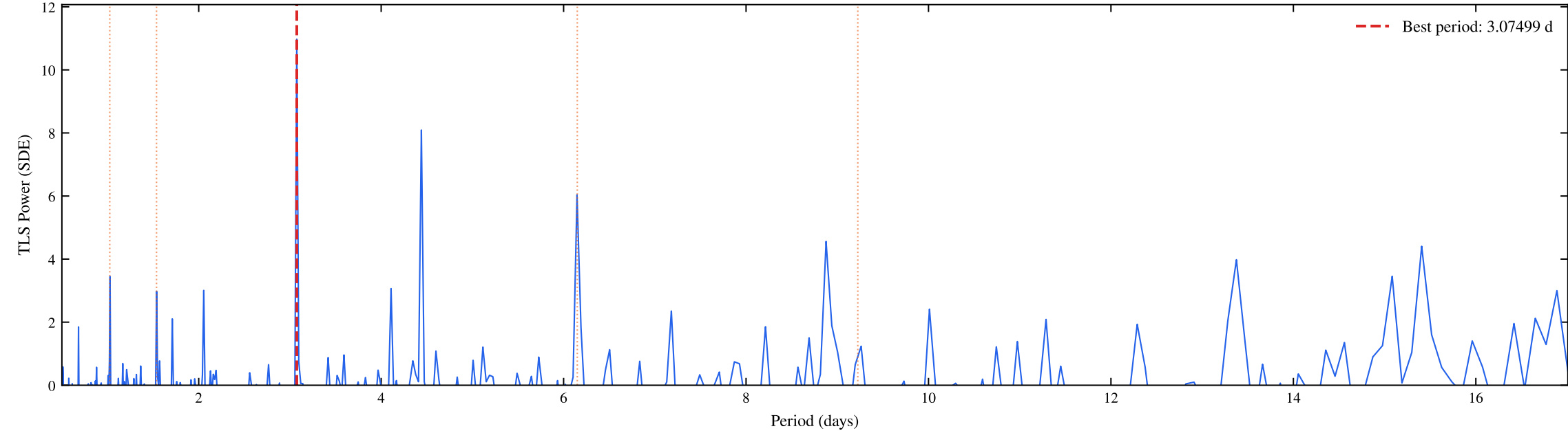
TIC 461867584 | Sectors: 36, 37 | TLS Periodogram (Planet 2 Search) (SDE = 10.97)
