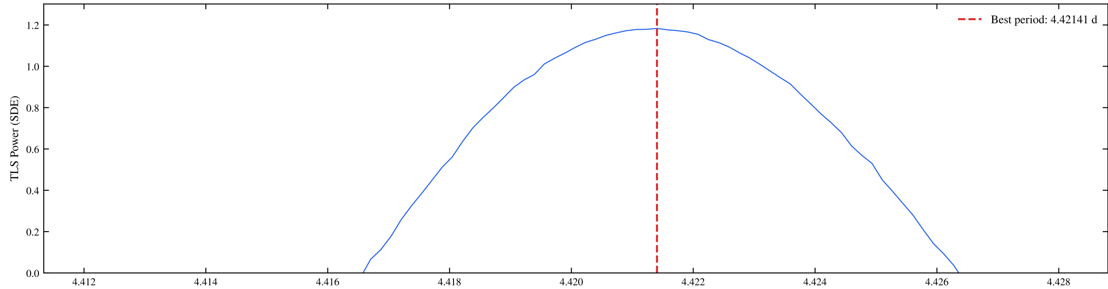
TIC 461867584 | Sectors: 36, 37 | TLS Periodogram (Planet 2 Search) (SDE = 10.97)
