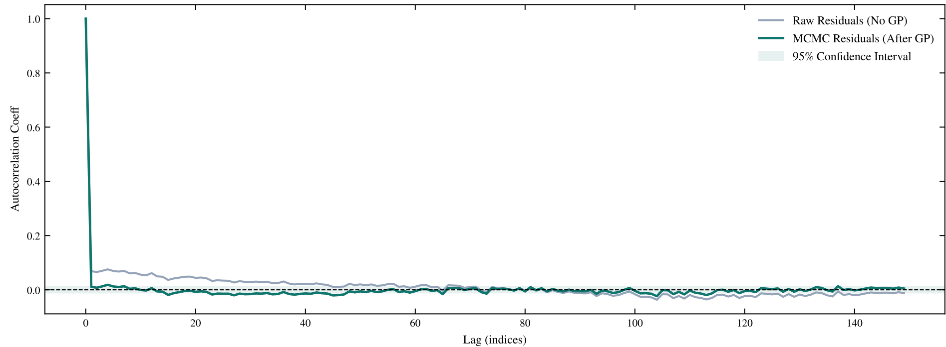
TIC 461867584 | Sectors: 36, 37 | GP Residuals Autocorrelation Function (ACF)
