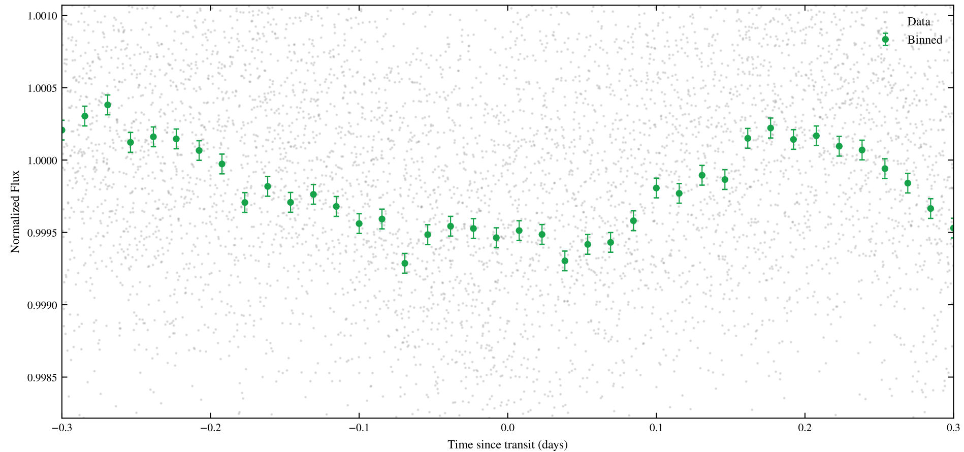
TIC 461867584 | Sectors: 36, 37 | Phase-Folded Transit (P = 3.07658 d)
