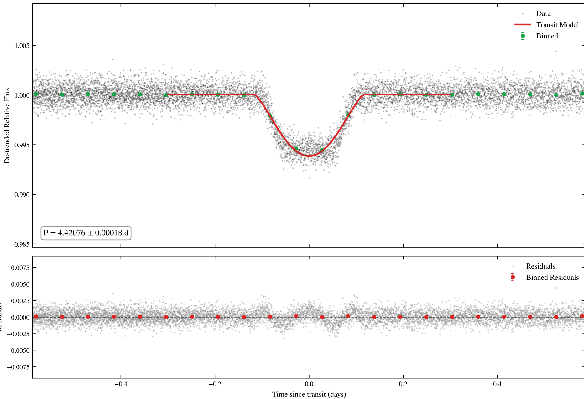
TIC 461867584 | Sectors: 36, 37 | Phased MCMC Fit - Planet 1
