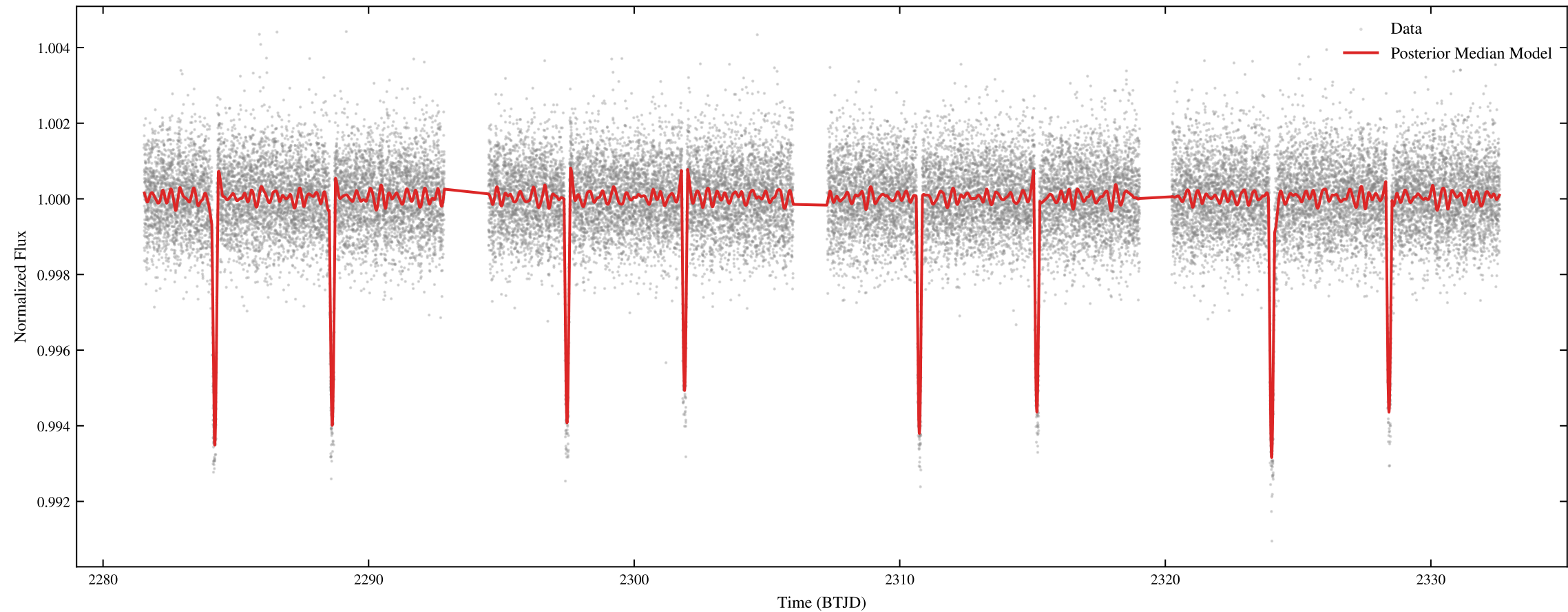
TIC 461867584 | Sectors: 36, 37 | MCMC Posterior Predictive Check
