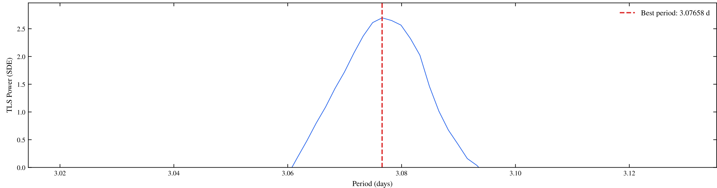
TIC 461867584 | Sectors: 36, 37 | TLS Fine Periodogram (SDE = 2.70)
